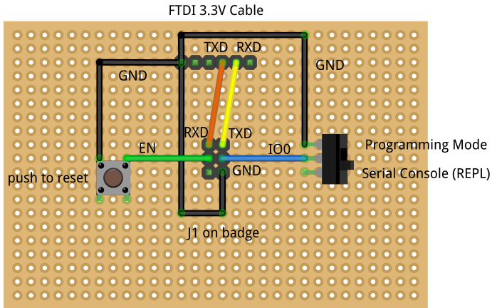
2018 Open Hardware Summit badge adapter board for J1 header for programming mode and serial console (MicroPython REPL) https://oshwabadge2018.github.io
