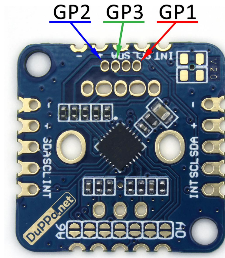
Figure 1.12: GP pins pinout
