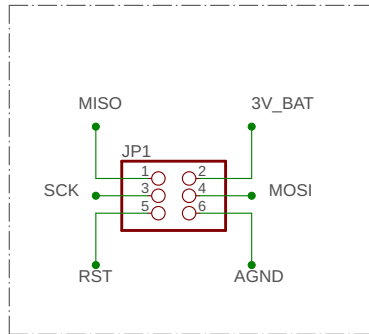
Standard ICSP Header
