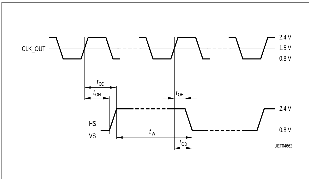
Timing Diagram 2
