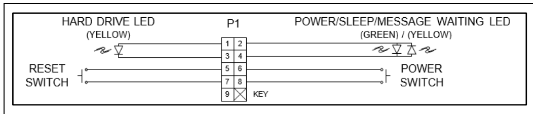
Figure 4-1. Switch/LED Cable
