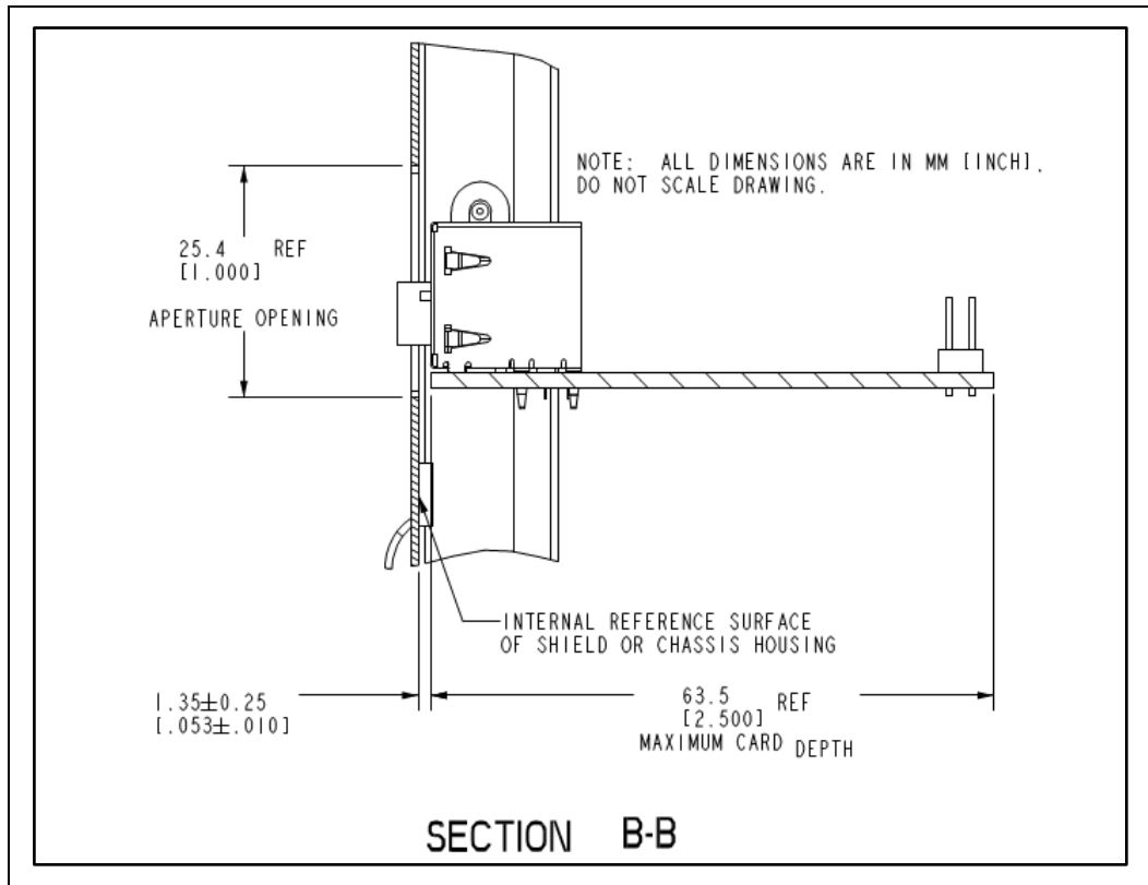
Figure 5-2. Front Panel I/O Interface Board Placement Recommendations
