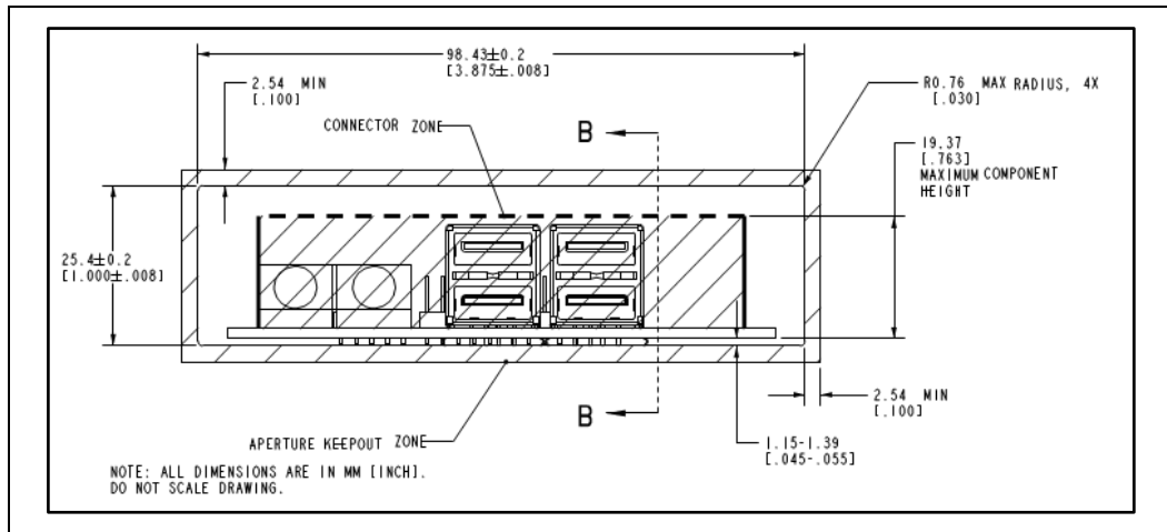
Figure 6-2. Front Panel I/O Interface Board Placement Recommendations
