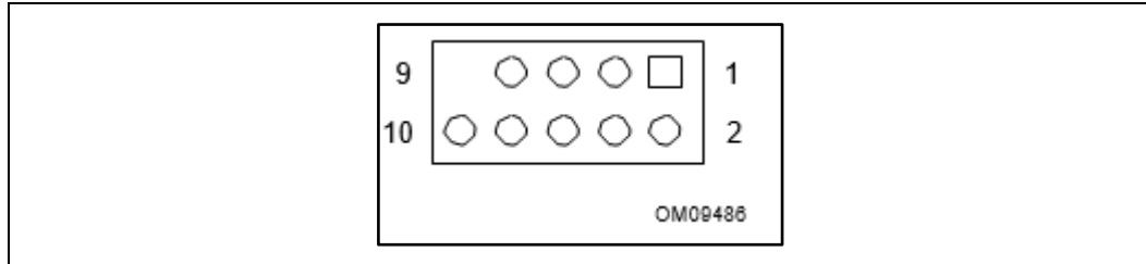
Figure 3-2. Front Panel IEEE-1394 Connector
