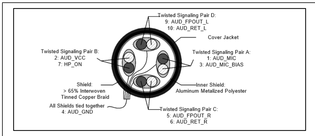
Figure 4-3. Audio Cable Cross-section
