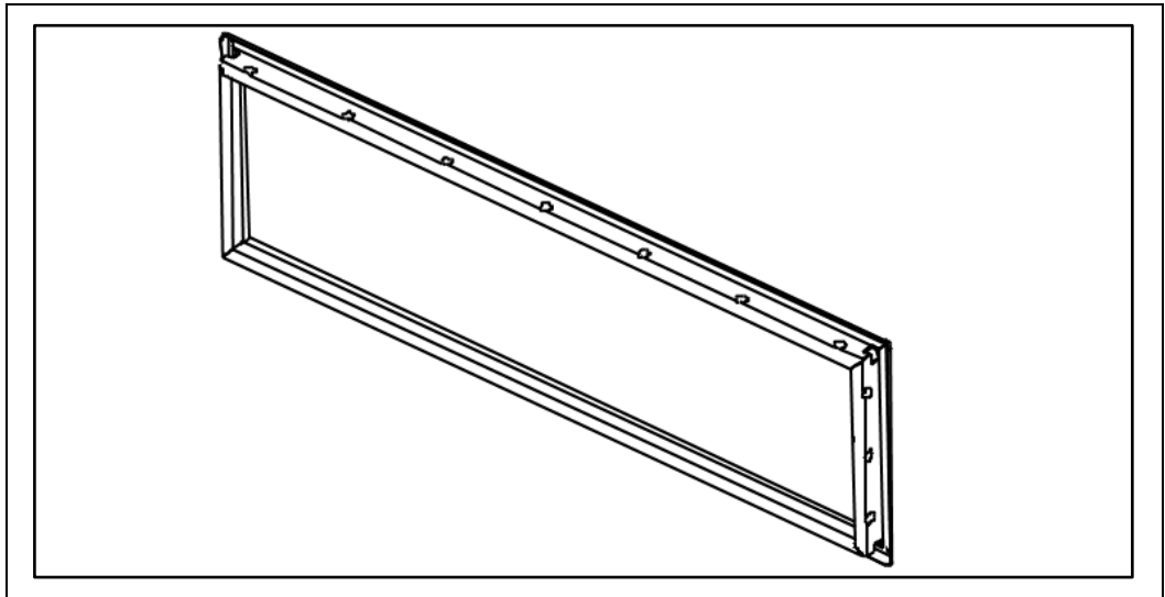
Figure 6-3. Front Panel I/O Shield Reference Design
