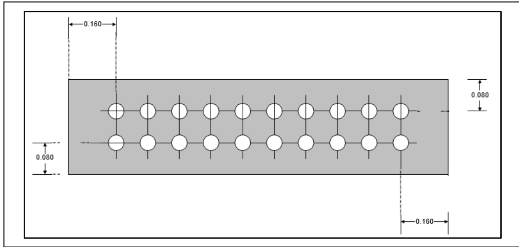
Figure 8-3. LPC Debug Connector Keep-Out Zone
