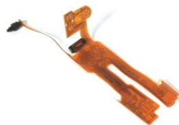
The flex circuit solution: A single circuit with 7 stiffeners and 2 connectors provides all the needed interconnects.
