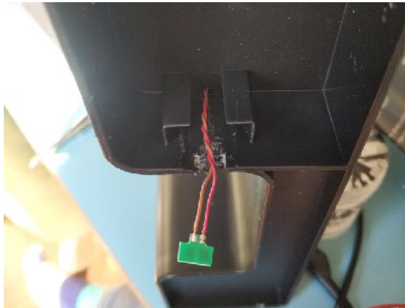
Solder on the back of the contacts, then twist and glue in place
