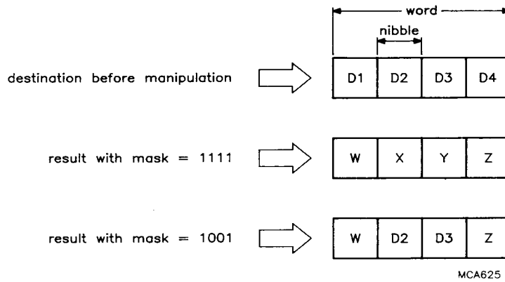
Fig.36 Mask example.
