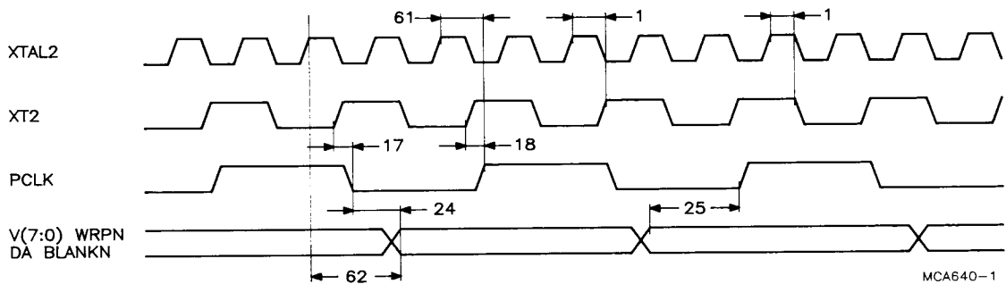
Fig.46 Pixel output timing.
