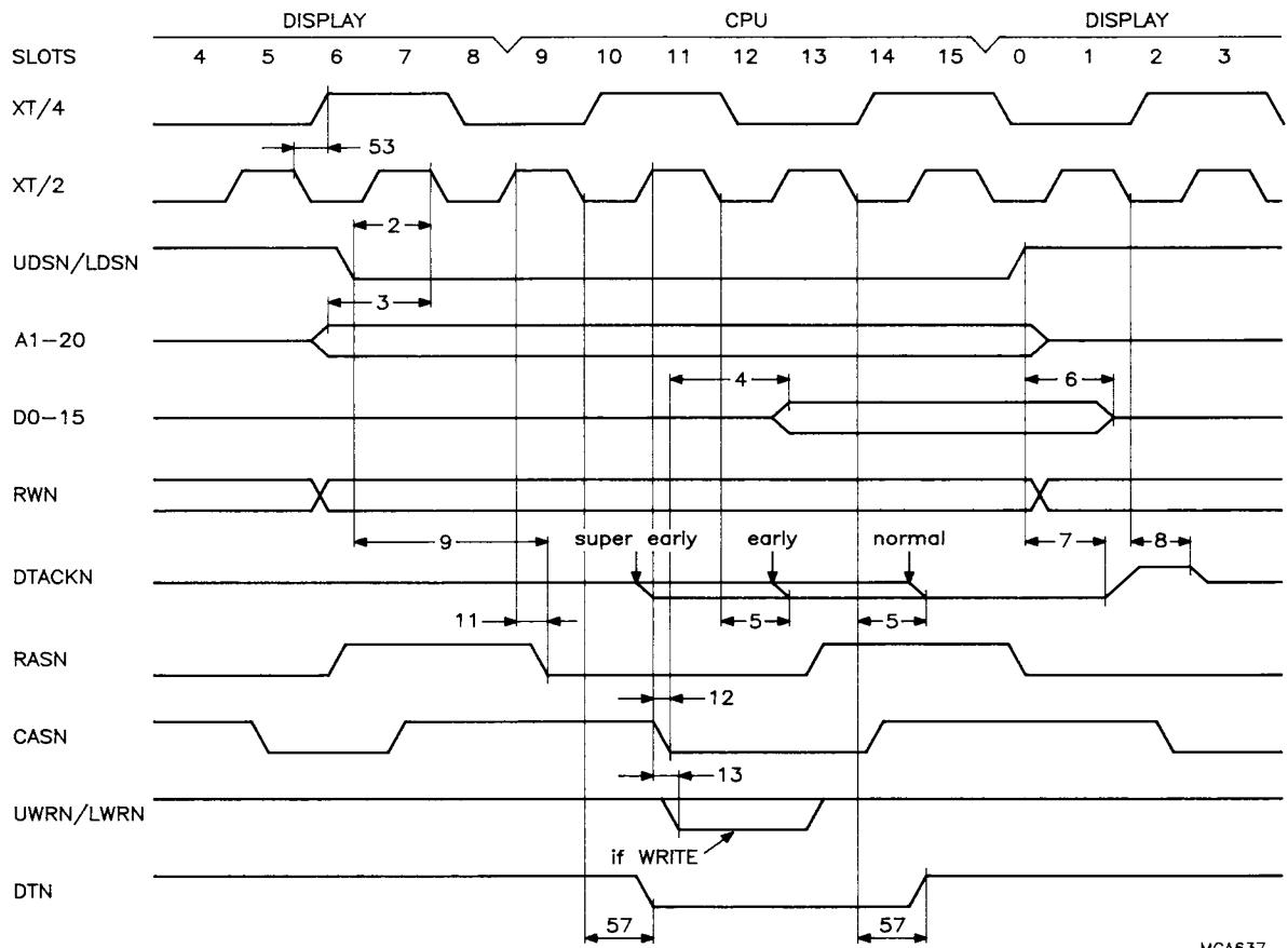
Fig.42 CPU <-> memory access in FAST mode.
