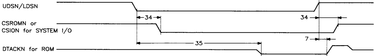
Fig.51 CSROMN and SYSTEM I/O timing.
