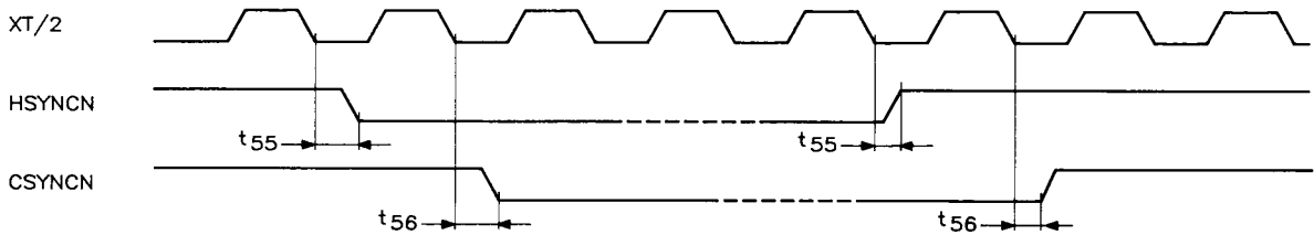
Fig.52 Synchronisation Timing.
