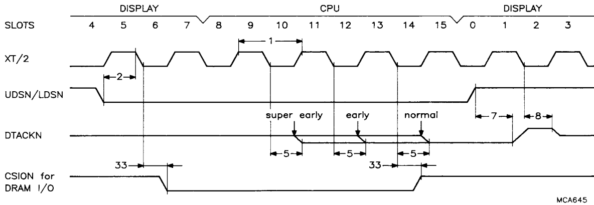
Fig.50 CSION timing in SLOW mode for a DRAM I/O access.
