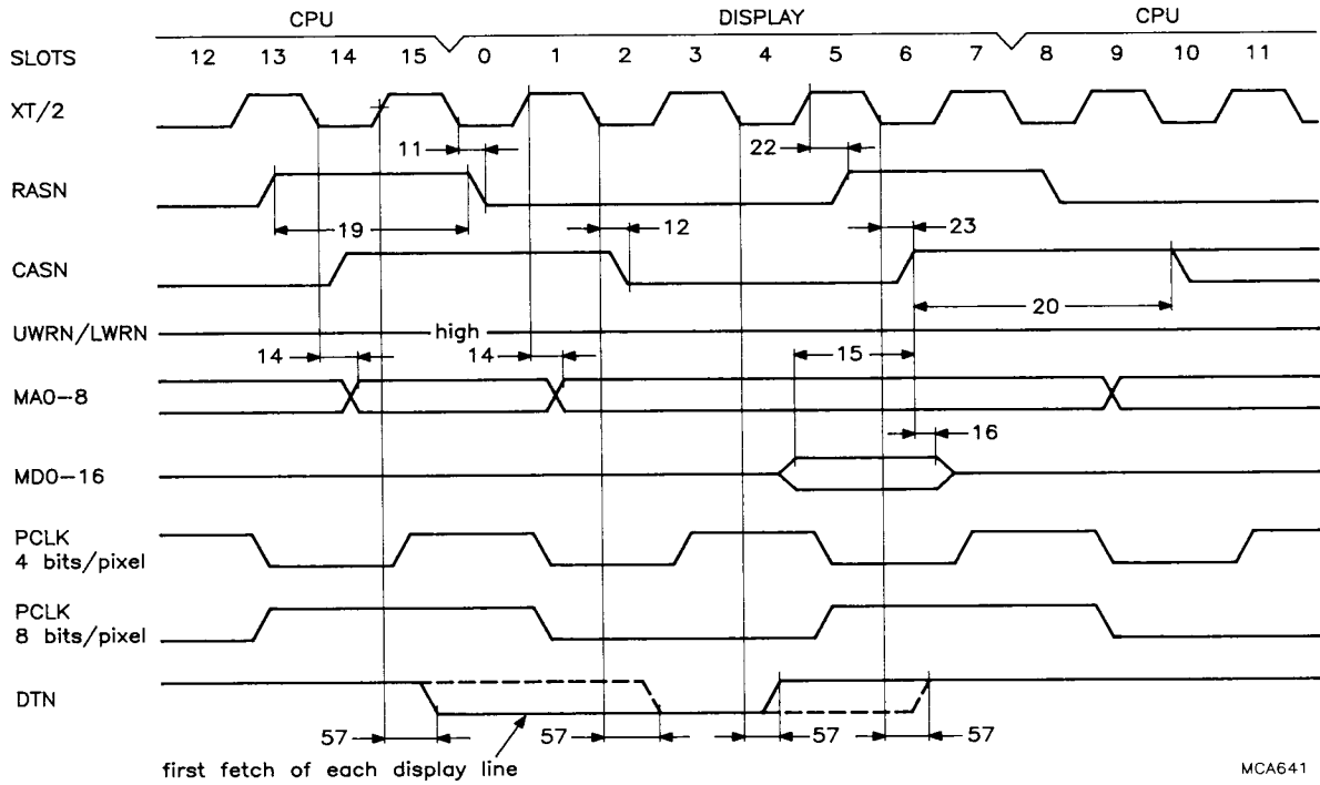
Fig.45 Display cycle in NORMAL mode.
