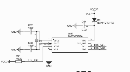
RTC
