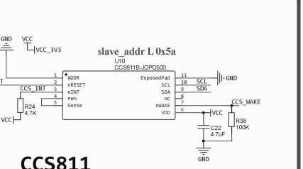
CCS811
