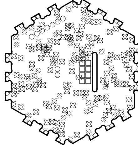
Drill Drawing View (Scale 1:1)
