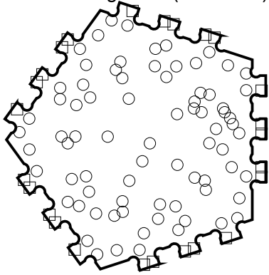
Drill Drawing View (Scale 1:1)
