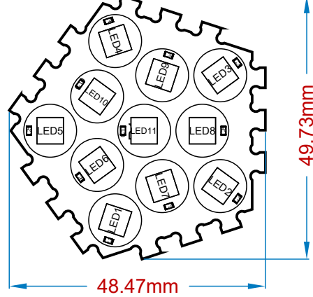
View from Top side (Scale 1:1)
