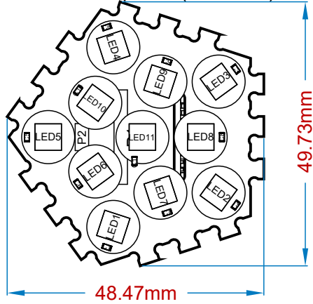
View from Front side (Scale 1:1)
