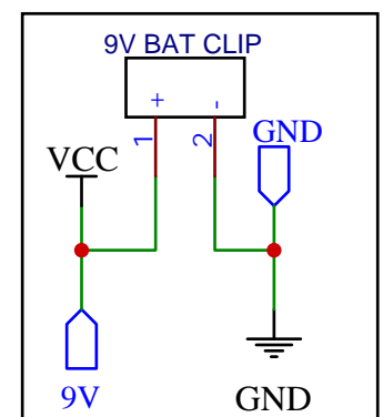
9V AND GROUND
