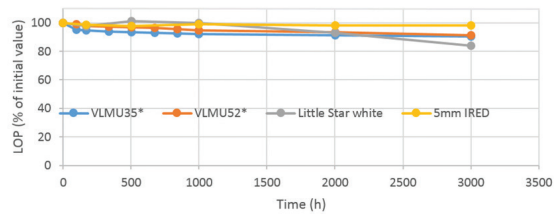
LIFETIME AT MAXIMUM JUNCTION TEMPERATURE
