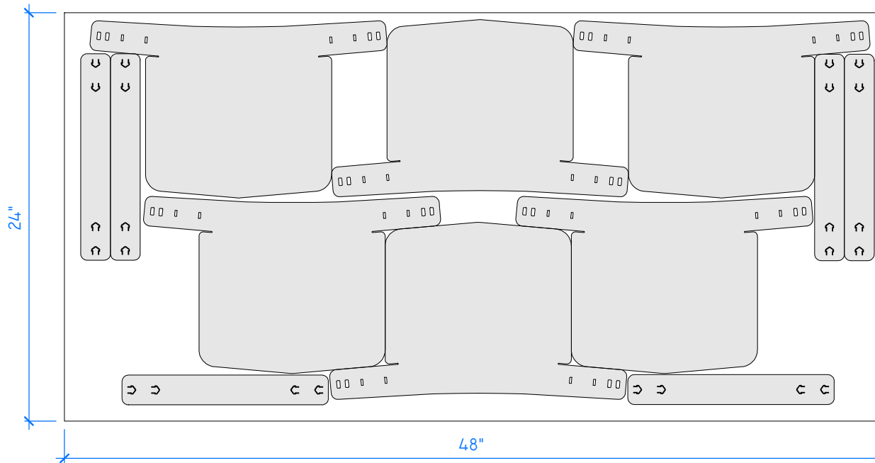
2 NESTED ON 2'X4' SHEET 3/4" = 1'-0"
