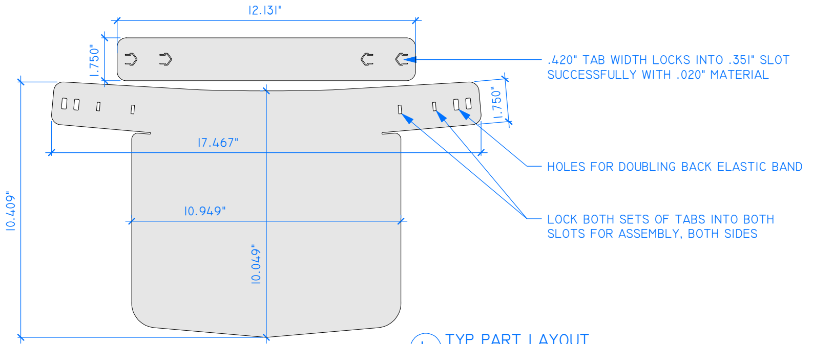
1 TYP PART LAYOUT 3" = 1'-0"
