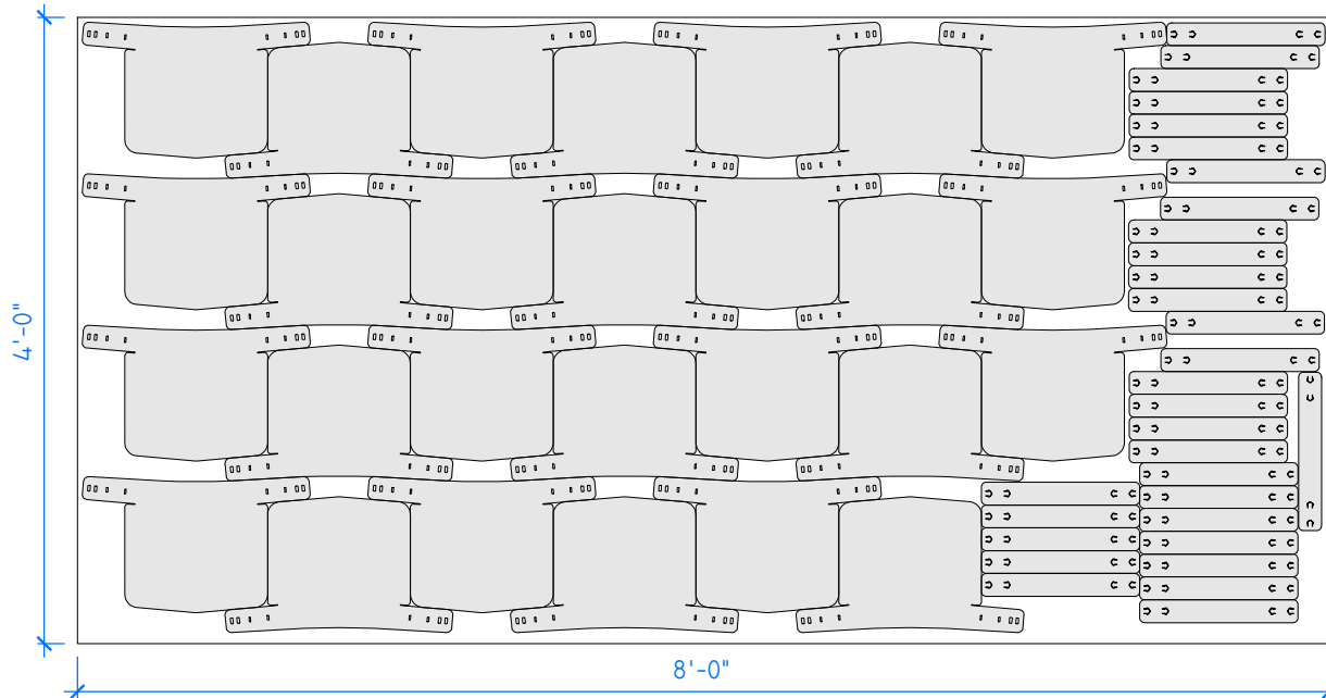
2 NESTED ON 4'X8' SHEET 3/4" = 1'-0"
