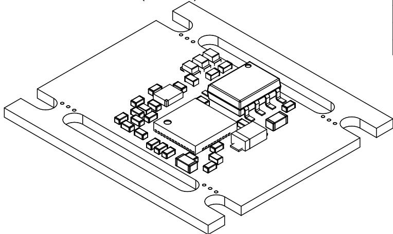
View from Front side (Scale 3)
