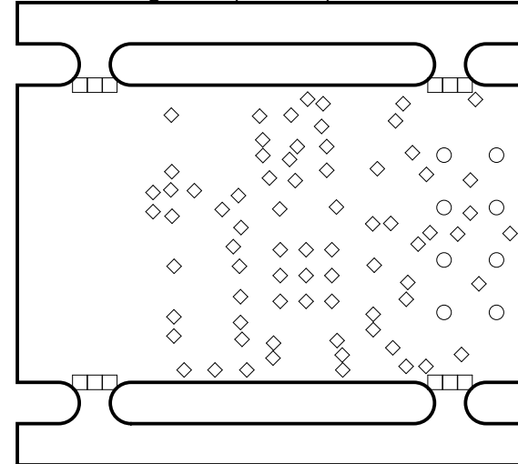
Drill Drawing View (Scale 3)
