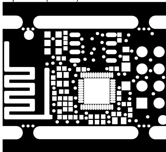
Top Solder (Scale 3)
