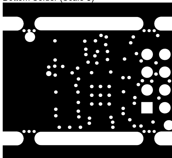
Bottom Solder (Scale 3)
