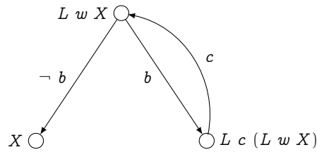
Fig. 10.6. Control-flow graph for WHILE\ b\ DO\ c
