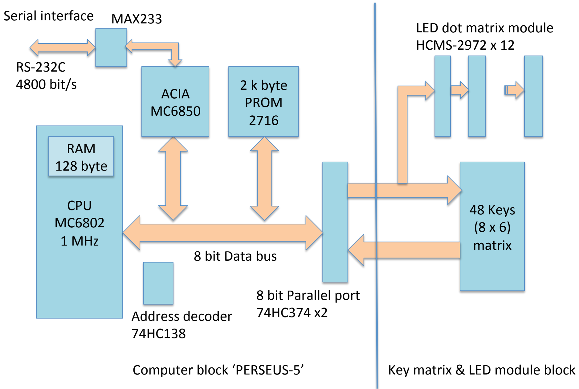
Fig 1 6802 Serial Terminal hardware block diagram
