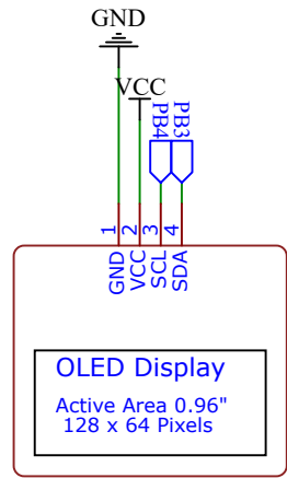
DY2 guki_OLED_DISPLAY_0.96*2019
