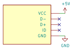
A2 USBBreakoutModule J2 USBBreakoutModule-Header-5POS
