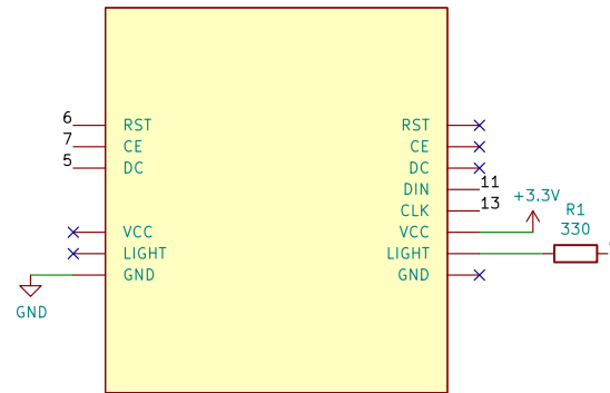
A4 Nokia5110LCD J6 Nokia5110LCD-TopHeader-8POS J9 Nokia5110LCD-BottomHeader1-3POS J10 Nokia5110LCD-BottomHeader2-3POS
