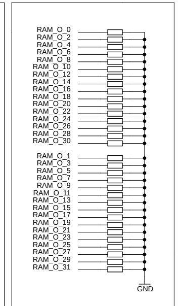
Pull-down resistors
