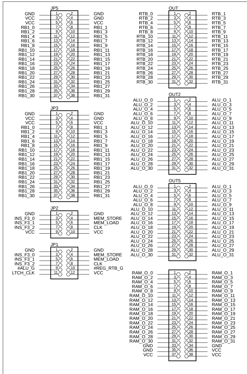
RTB_IMM_MUX and latch (SEL. 1)
