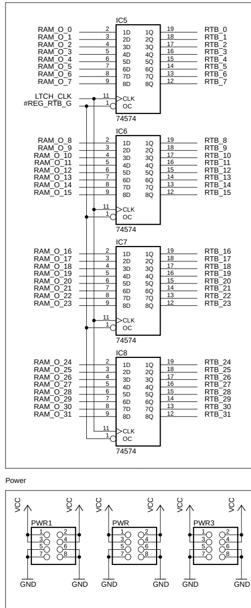
RTB_IMM_MUX and latch (SEL. 1)
