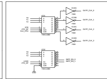
Output registers
