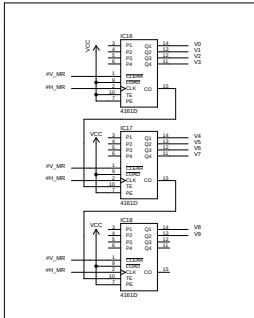
Vertical logic
