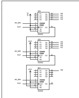
Horizontal logic
