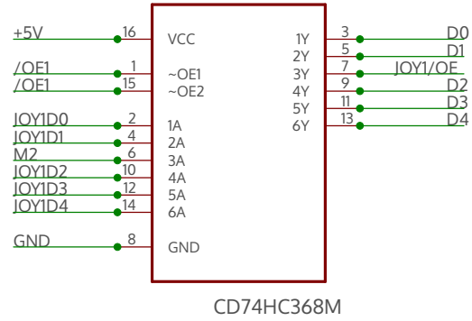
U7-HEXBUFFER1
