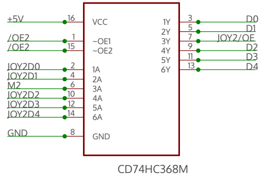
U8-HEXBUFFER2
