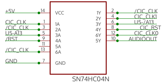
U9-HEXINVERTER1
