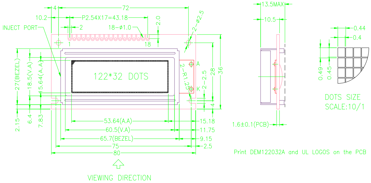
Figure 2. Dimensional outline
