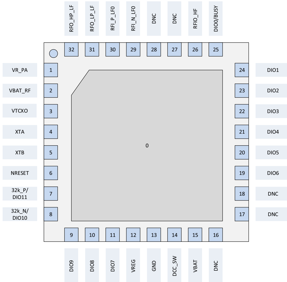
Figure 2-1: LR1121 Pinout
