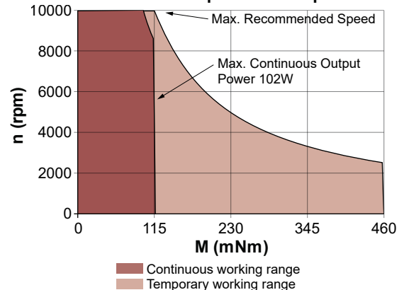
No Load Speed vs. Torque
