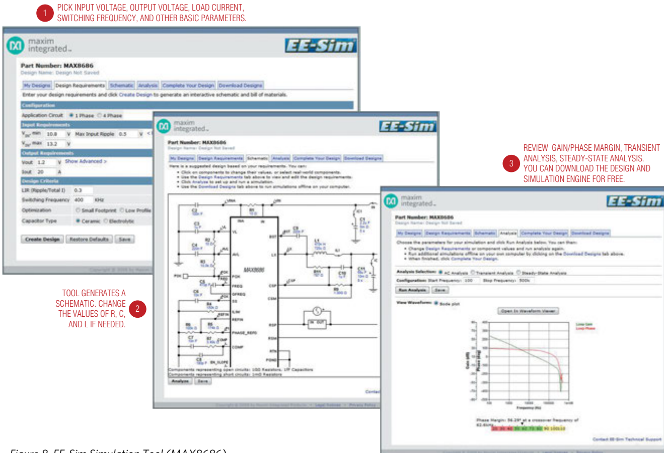
Figure 8. EE-Sim Simulation Tool (MAX8686)
