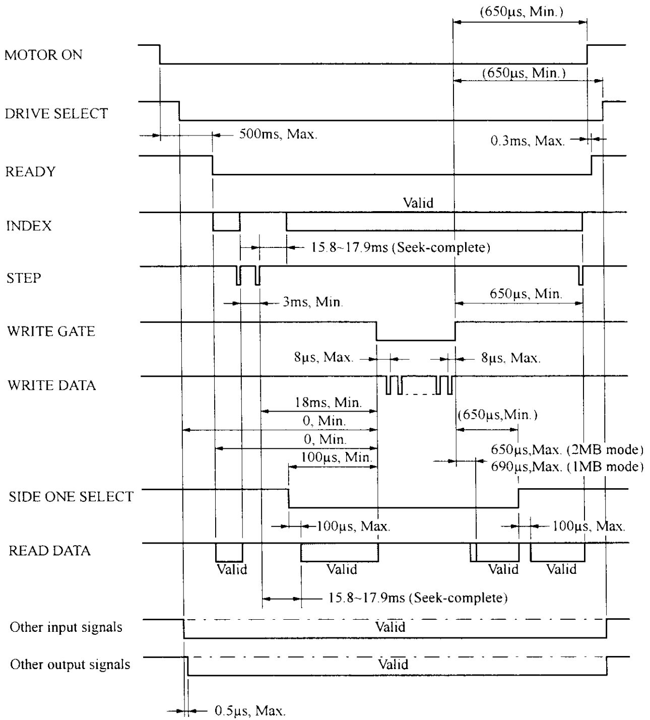
(Fig. 9.3-1) Read/Write operation timing
