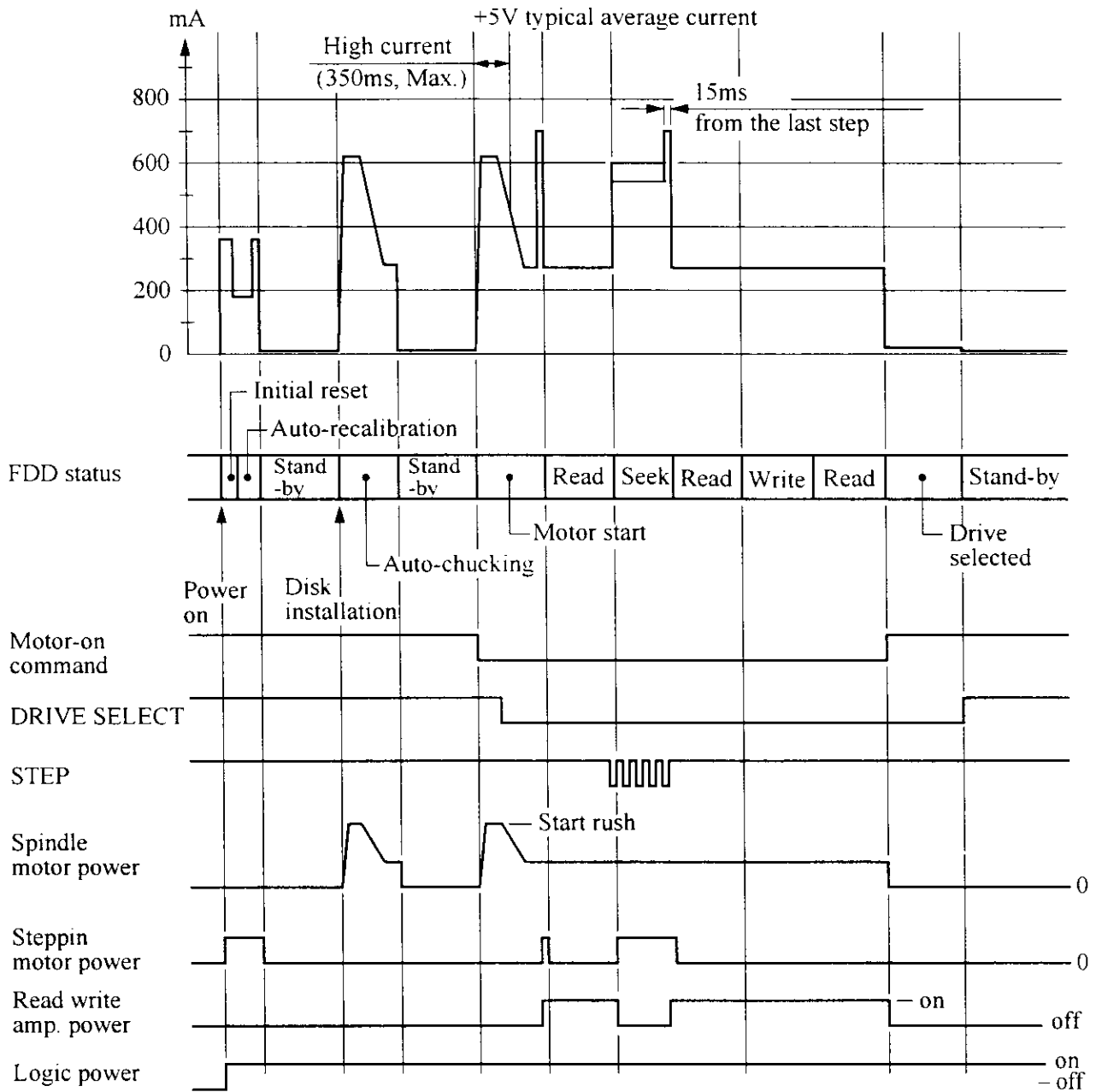
(Fig. 9.4-1) Typical average current profile
