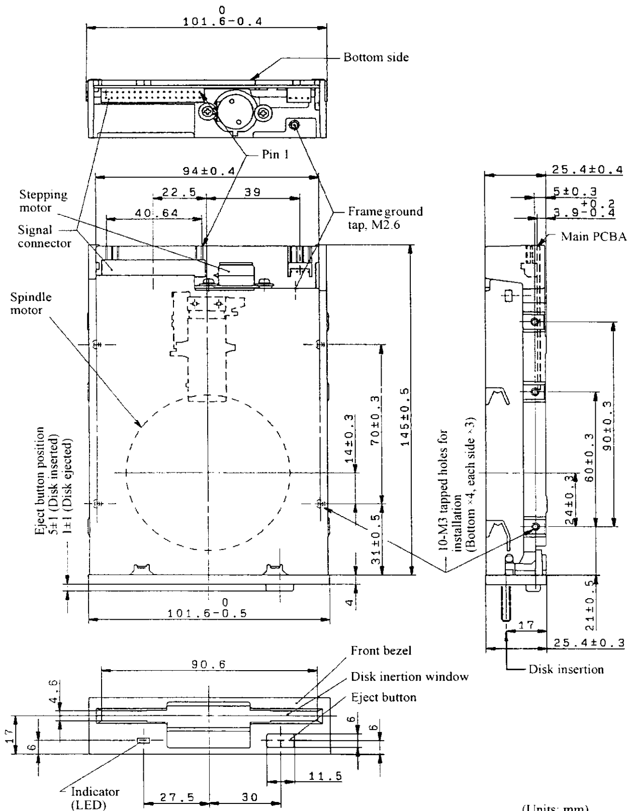
(Fig. 3-1) FDD external view
