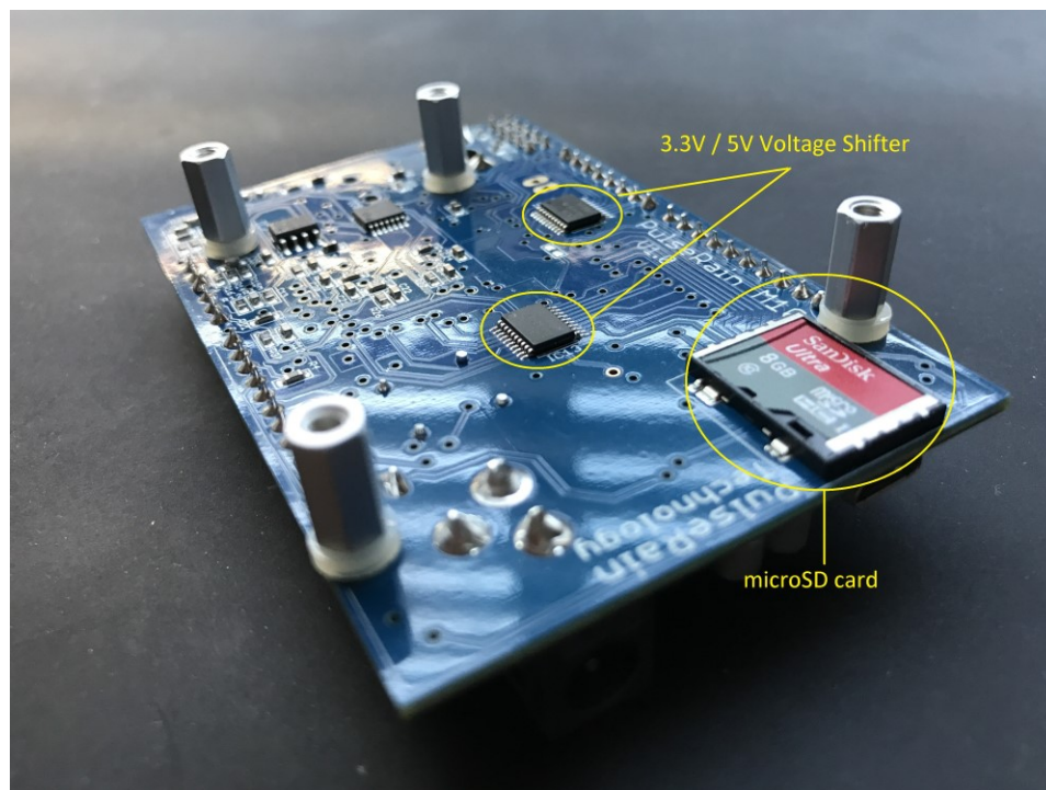
Figure 1-3 The Bottom View of M10
