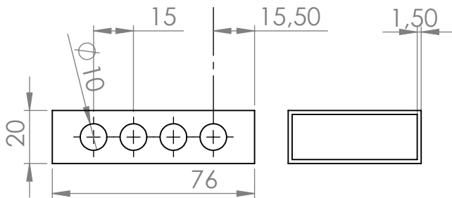
VIEW Top
