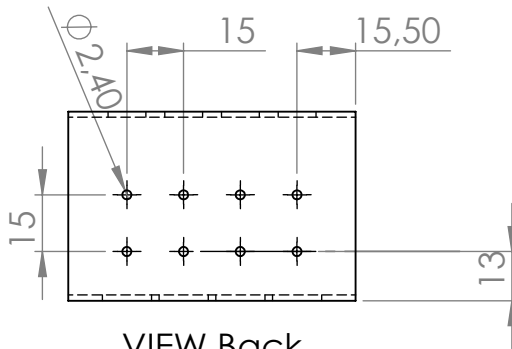
VIEW Back
