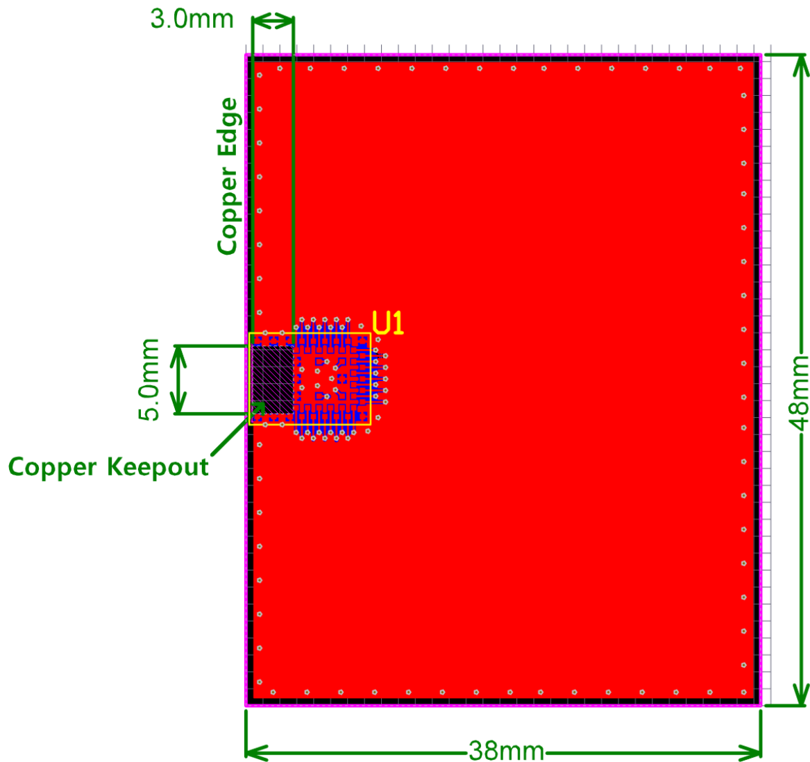
Figure 15 – BMD-350 Recommended RF Layout
