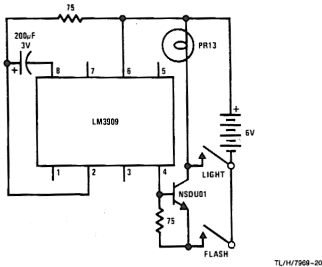
Emergency Lantern/Flasher
