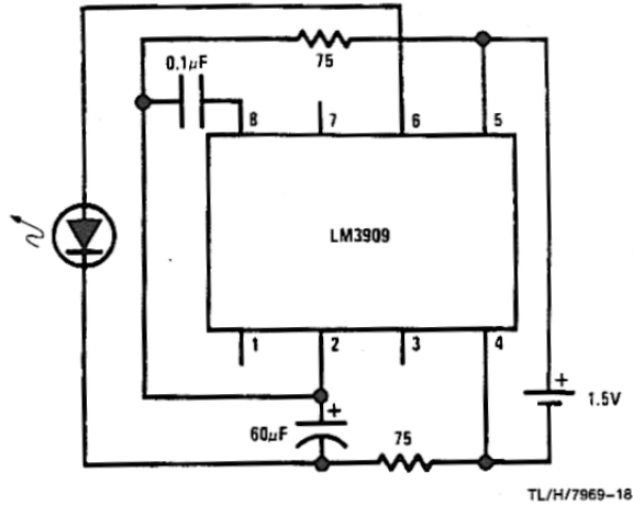
LED Booster
