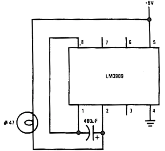
Incandescent Bulb Flasher
